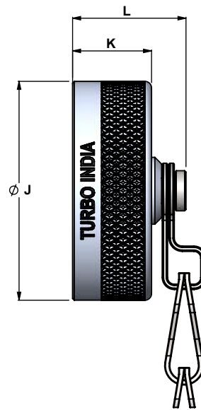
63 - RECEPTACLE COVER
