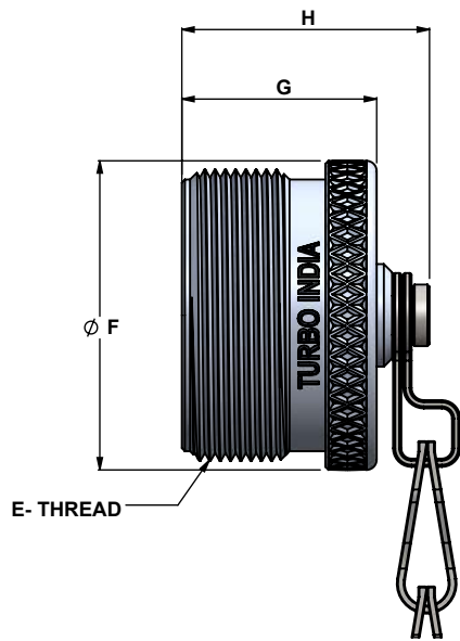
62 - PLUG COVER
